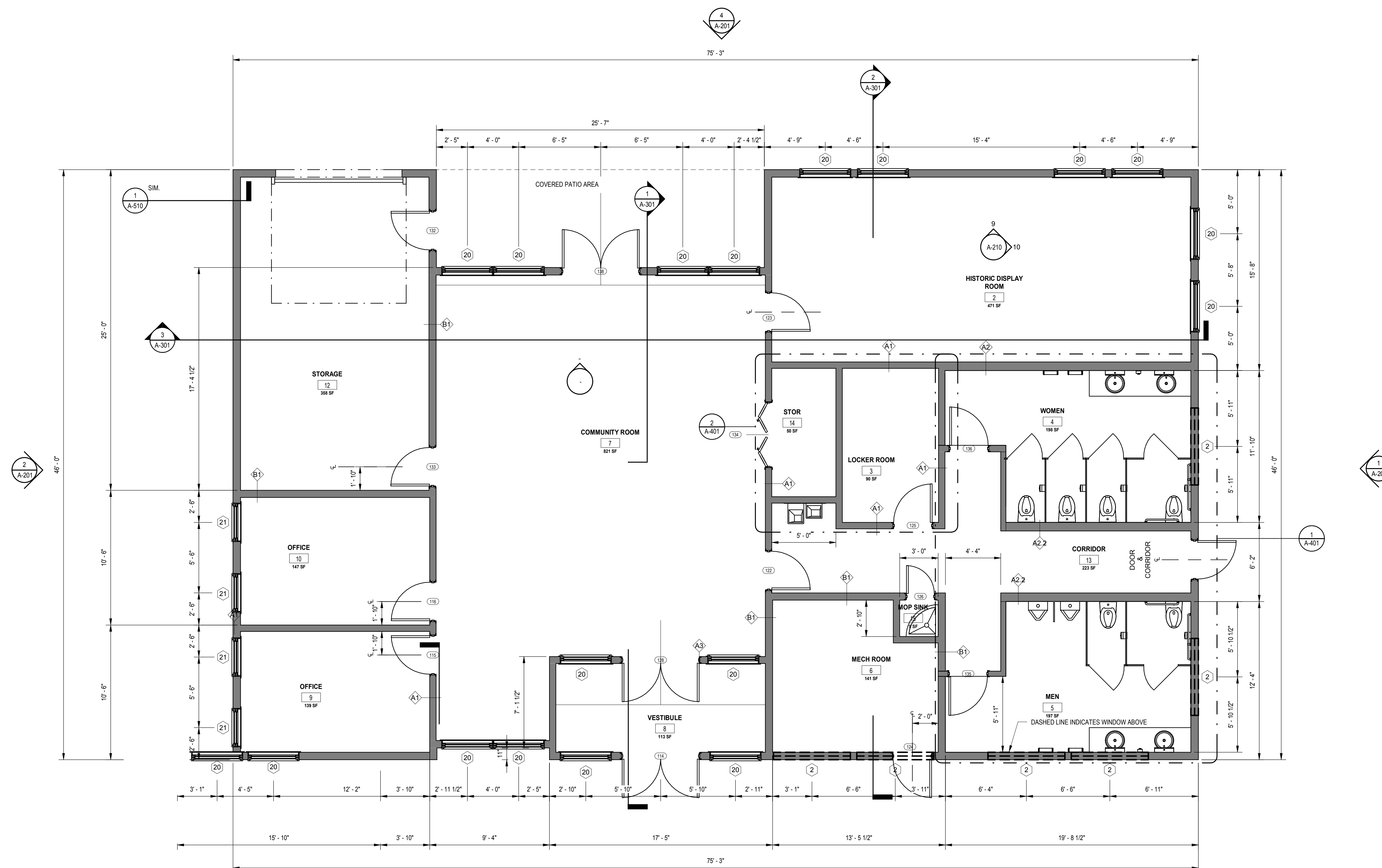
1 PLAN VIEW A-101 SCALE: 1/4" = 1'-0"
